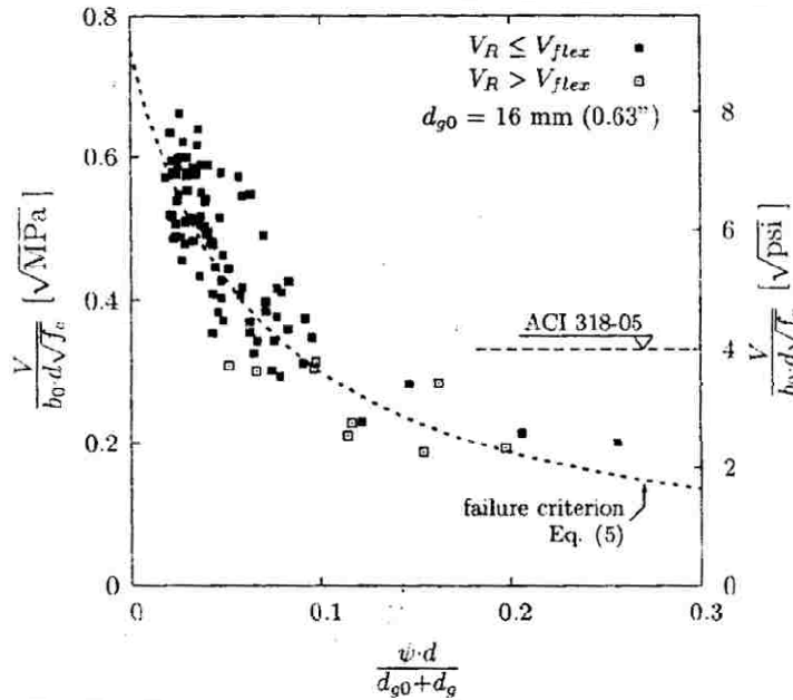
Figure 4-18 Punching shear strength as a function of slab rotation (Muttoni, 2008)
