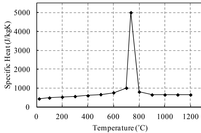
Figure 2-10 Steel specific heat
