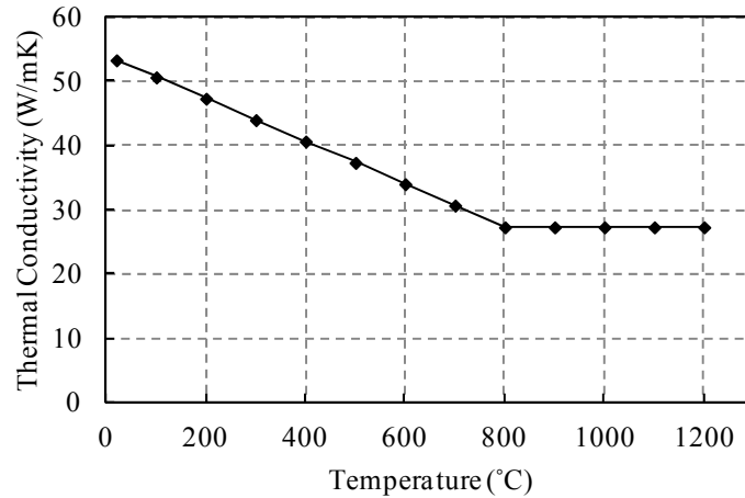
Figure 2-9 Thermal conductivity of steel
